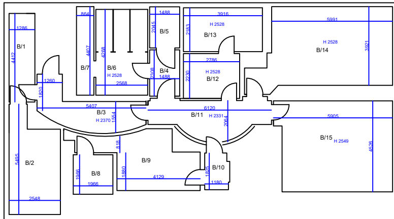
Basement
