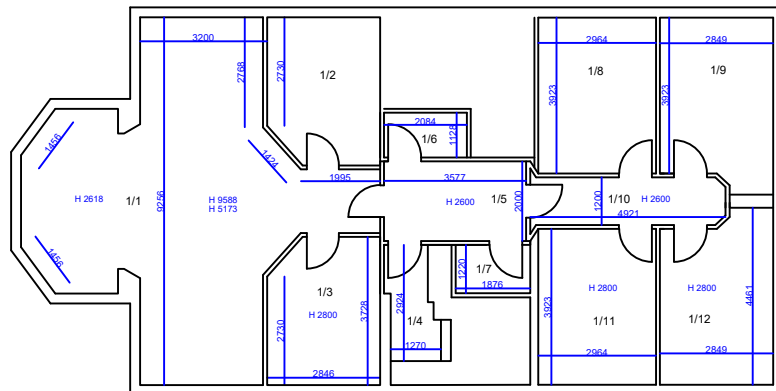
1st Floor
